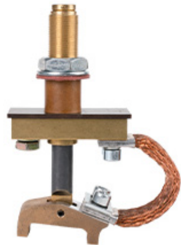
TSA 350 with bronze brush and connector
