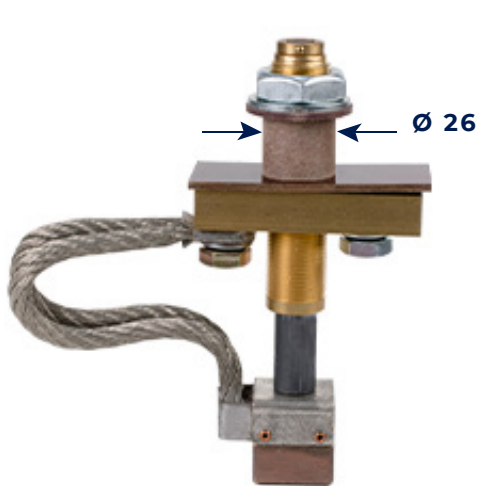
TSA 200 with carbon brush and connector
